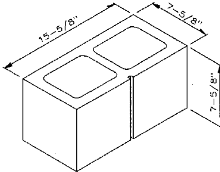
8-8-16 Scored One Side Standard CMU
